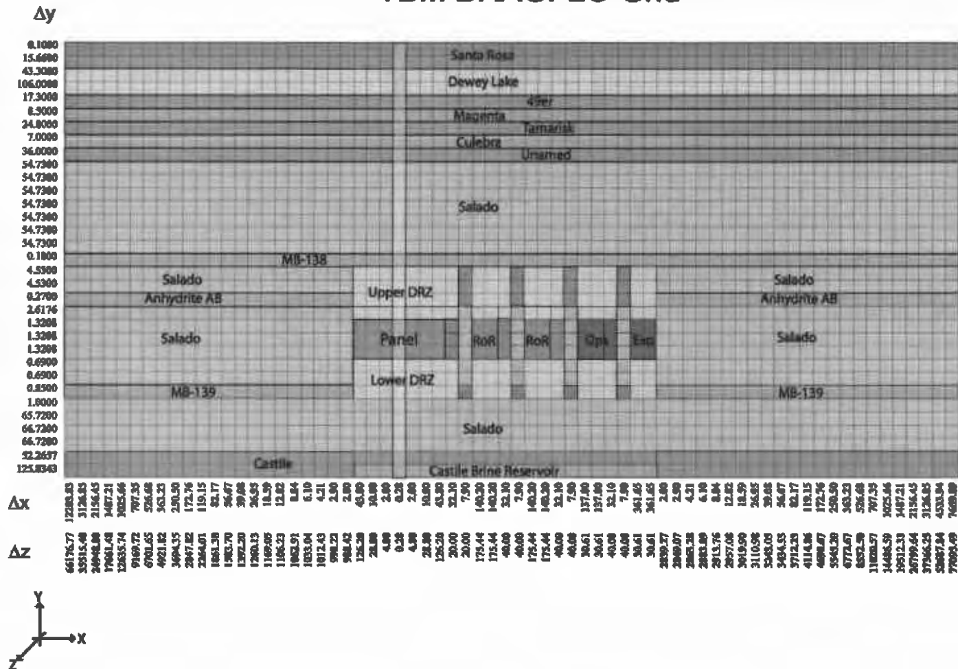
Figure 2. Technical Baseline Migration (TBM) logical BRAGFLO grid.
