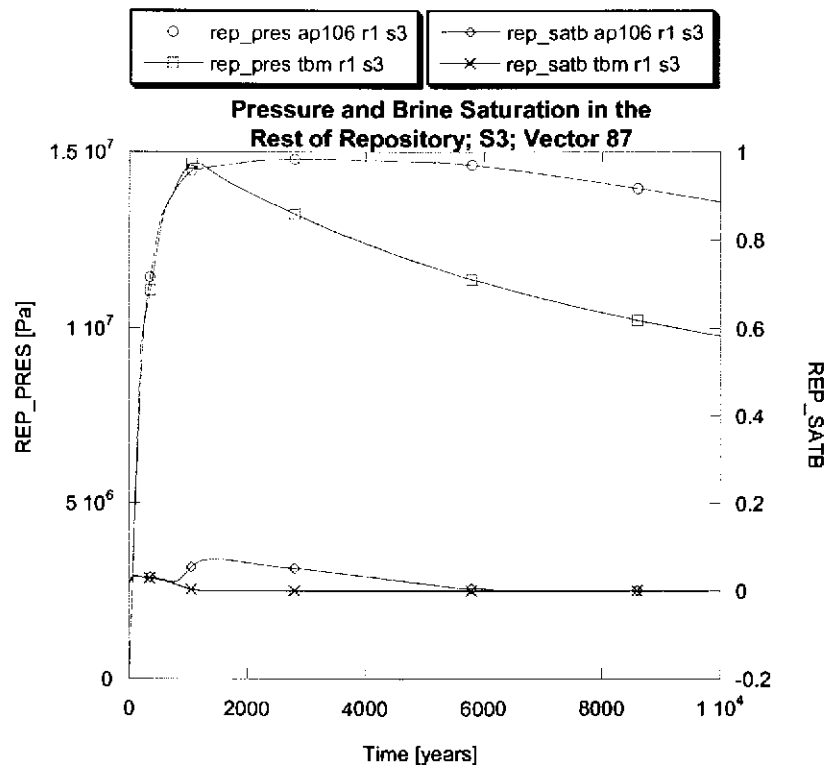
Figure 18. Detailed plot of pressure and brine saturation time histories for vector 87; S3
